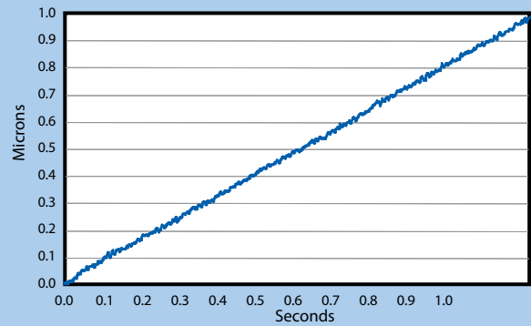
Velocity Ripple
