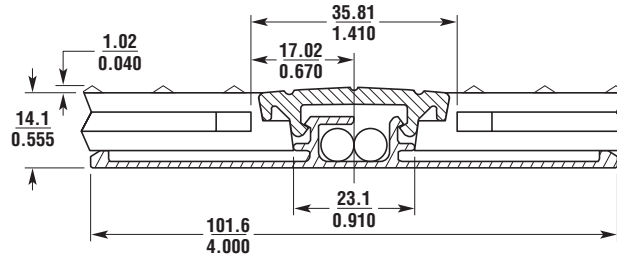
Figure 4-8 Picture Below Shows Joining Trim NOT Stepped On
