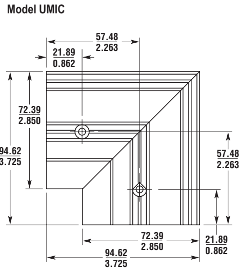
Figure 4-2 Dimensions and Installation Information for 2-Part Aluminum Base, PVC Cover with Molded Corners
