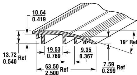
Figure 4-5 Dimensional Information (Trim Only)
