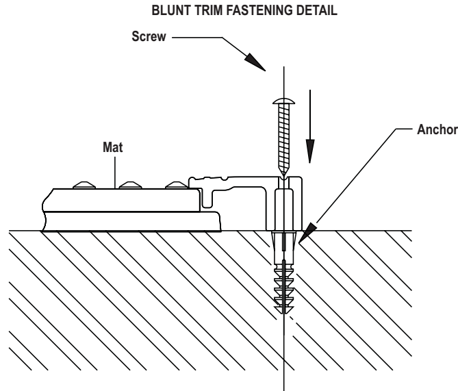
Figure 4-6 Blunt Trim Installation Information
