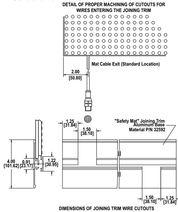
Figure 7-5 Joining Trim Wire Cutouts
