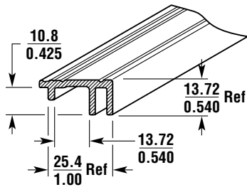
Figure 4-7 Blunt Trim Dimensional Information
